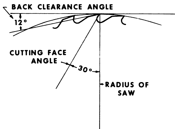
Figure 10-2. Design of tooth and gullet, showing proper clearance and hook angles for solid-tooth saws.
